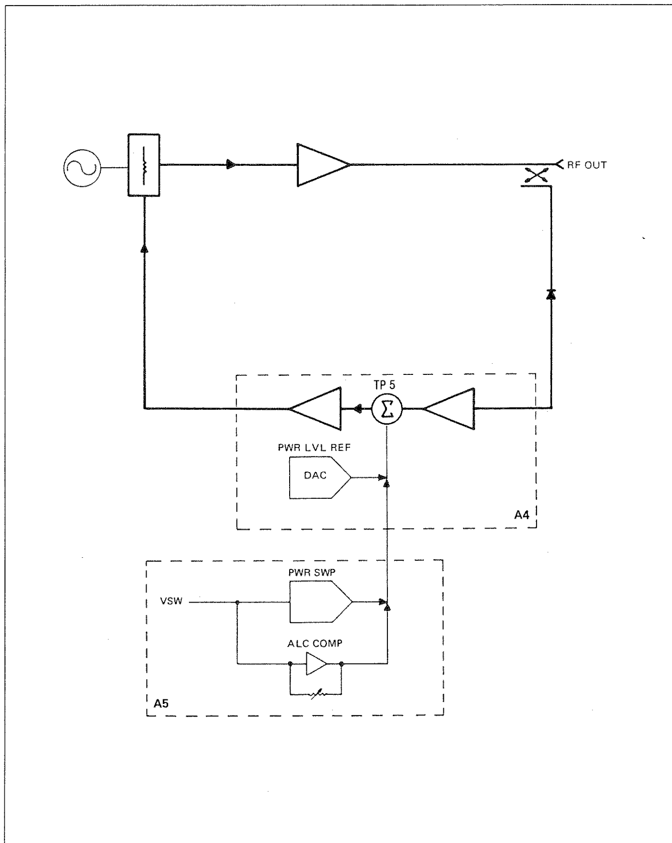
Figure 8-30. Simplified ALC Block Diagram
