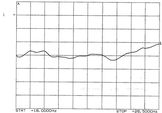
Figure 5-21. Trace After First Breakpoint and Slope Adjusted
