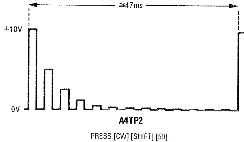
Figure 8-26. DAC Test
